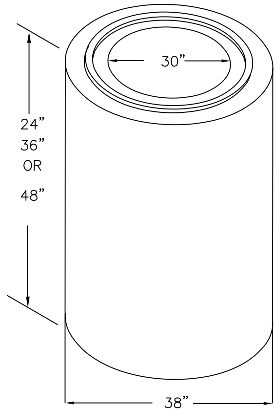
24" RISER H-20 R2430H
