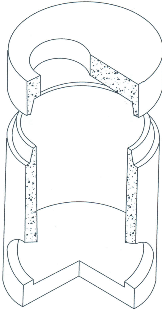
DRAIN MANHOLE 5' DIAMETER
