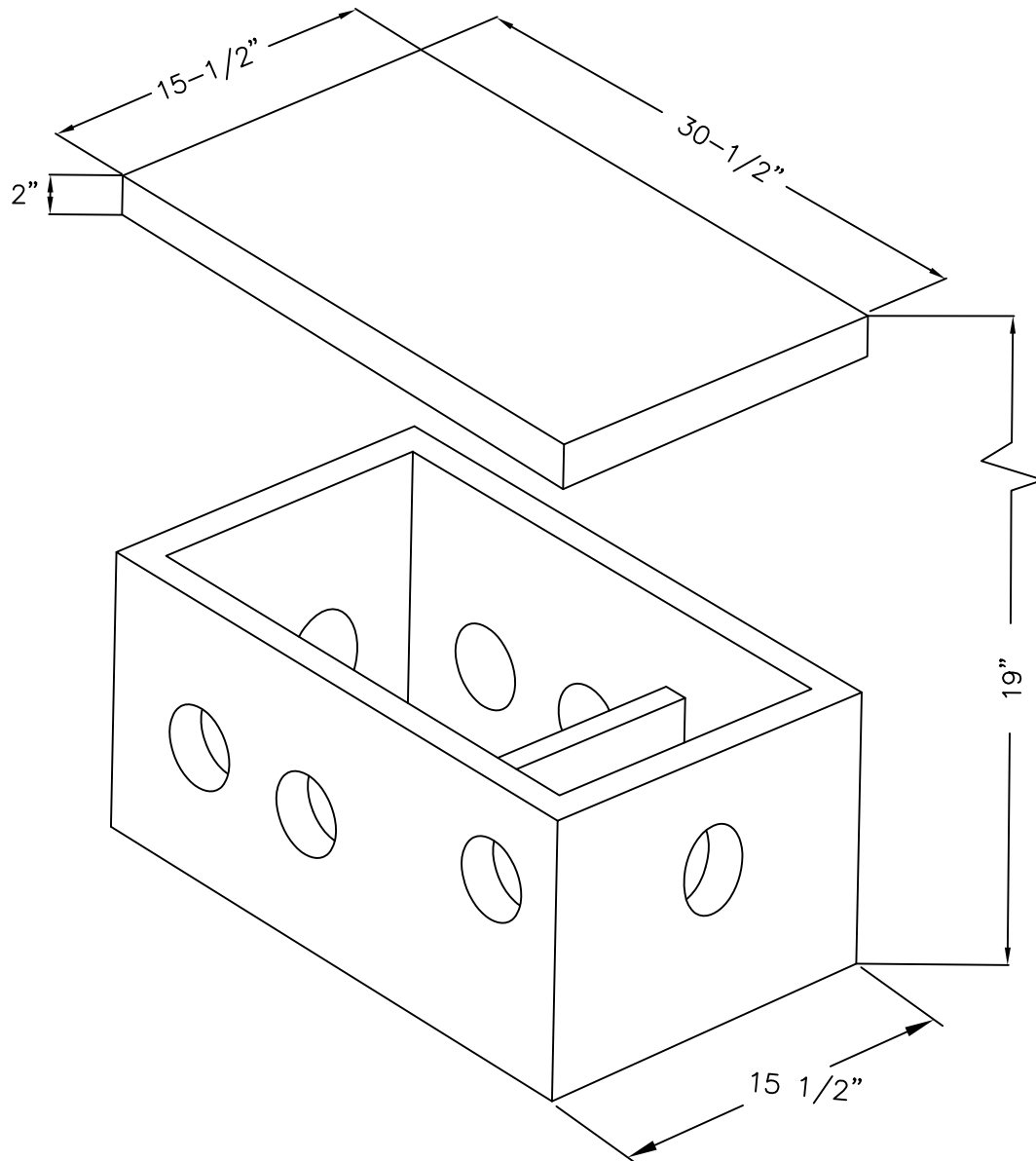
DB-5B DISTRIBUTION BOX: 5 OUTLET WITH BAFFLE
