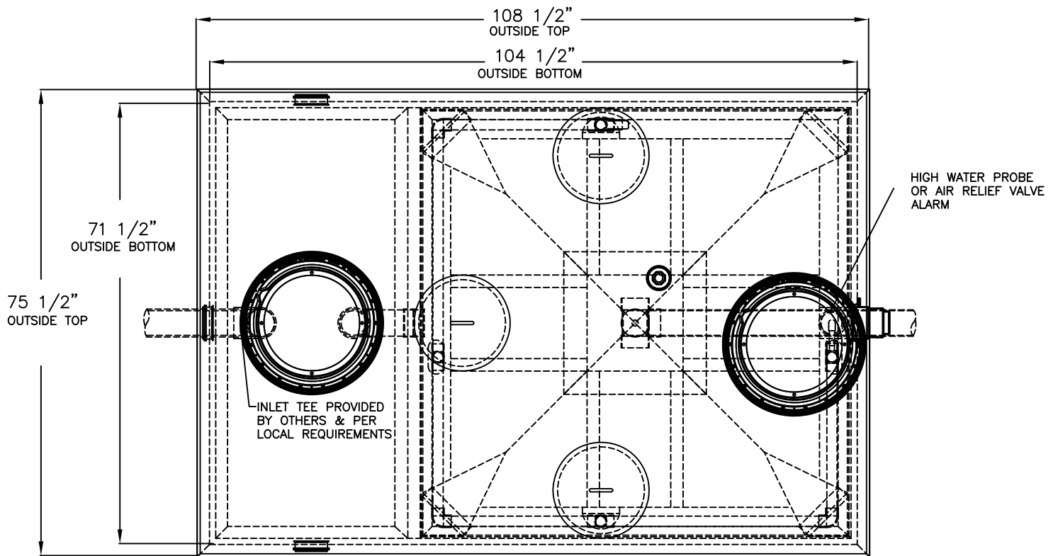
PLAN VIEW
